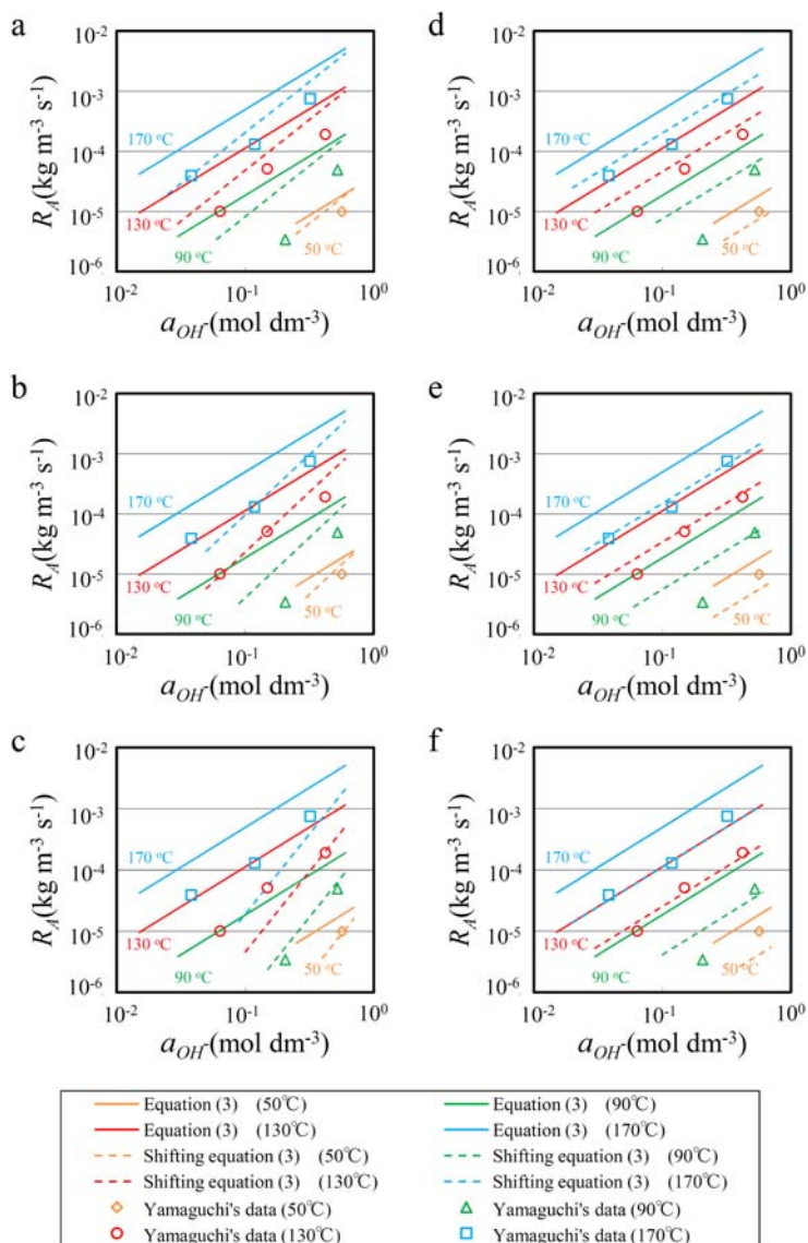
FIG. 7. Comparison between the dissolution rate of montmorillonite in the mixtures and the curves given by shifting equation 3: (a) by 0.05 \text{ mol dm}^{-3} ; (b) by 0.1 \text{ mol dm}^{-3} ; (c) by 0.2 \text{ mol dm}^{-3} ; (d) by shifting by 0.3 logarithmic units; (e) by 0.4 logarithmic units; and (f) by 0.5 logarithmic units.
