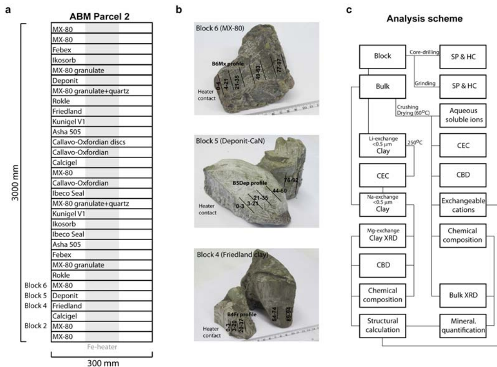
FIG. 1. (a) ABM parcel 2 experimental setup. (b) Photos of samples of the blocks on which the majority of analyses were done. Sampling and sample distance from the heater contact are given in mm. (c) Analysis scheme. Abbreviations: SP & HC = swelling pressure and hydraulic conductivity, CEC = cation exchange capacity, CBD = citrate-bicarbonate-dithionite extraction, XRD = X-ray diffraction.
