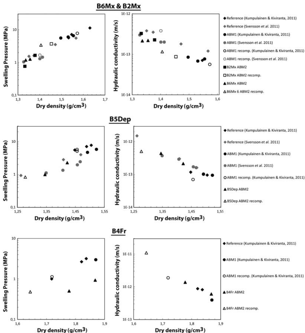
FIG. 8. Swelling pressure and hydraulic conductivity of drill-cored samples (filled symbols) and recompacted samples (open symbols) from the present study (ABM2) as a function of dry density. Reference samples (diamonds) and samples from previous studies (ABM1, circles) are shown for comparison with results in the present study (ABM2).
