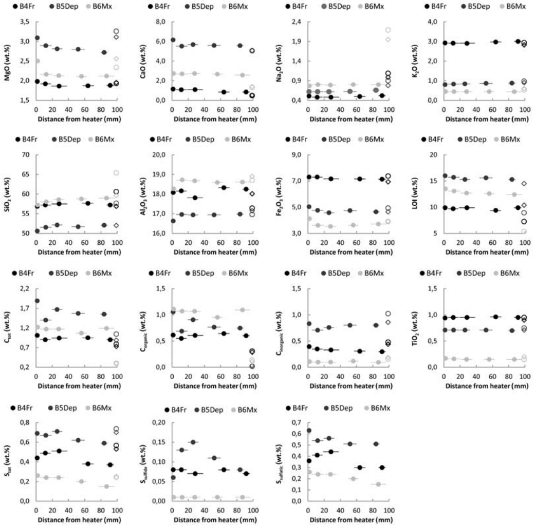
FIG. 5. Chemical compositions in horizontal profiles of the Friedland clay, Deponit CaN and MX-80 as a function of the distance from the heater. The open symbols are reference levels from Kumpulainen & Kiviranta (2010) (circles) and Svensson et al. (2011) (diamonds).
