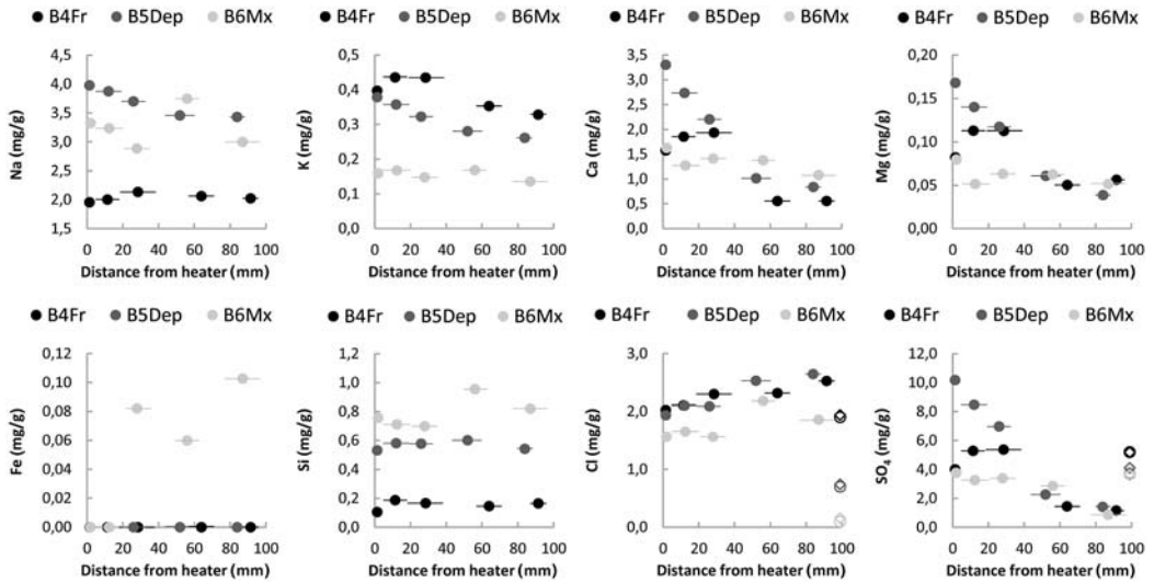
FIG. 2. Aqueous soluble ions as a function of the distance from the heater. Open symbols shown for Cl and \text{SO}_4 are reference levels from Muurinen (2010) (circles) and Svensson et al. (2011) (diamonds).
