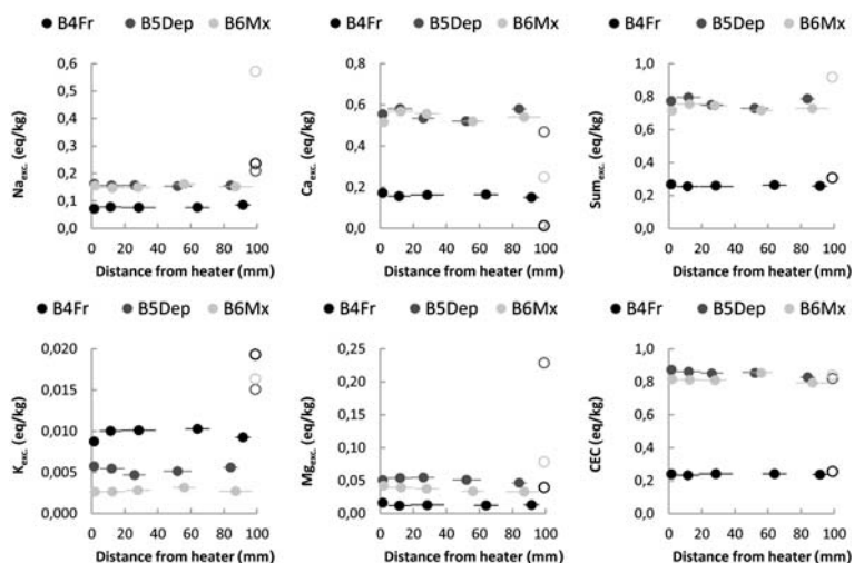
FIG. 4. Exchangeable cations and CEC values (as eq/kg of dry (105°C) mass) as a function of the distance from the heater. Open symbols are reference levels from Kumpulainen & Kiviranta (2011) (circles).
