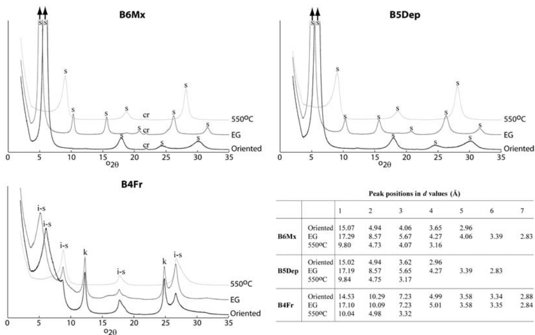
Fig. 7. XRD patterns, the minerals identified and peak positions for oriented clay fractions separated from samples at distances of 4–21 mm (B6Mx), 3–21 mm (B5Dep) and 3–20 mm (B4Fr) from the iron heater. Abbreviations: s = smectite, m = illite/mica, i-s = interstratified illite-smectite, k = kaolinite, cr = cristobalite, oriented = air dry sample, EG = ethylene glycol-solvated sample, 550°C = heat-treated sample.
