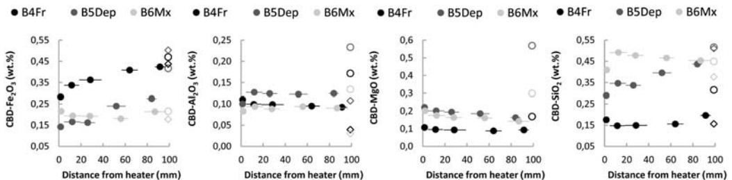
FIG. 3. CBD-extractable \text{Al}_2\text{O}_3 , \text{Fe}_2\text{O}_3 , MgO and \text{SiO}_2 as a function of the distance from the heater. Open symbols are reference levels from Kumpulainen & Kiviranta (2011) (circles) and Svensson et al. (2011) (diamonds).
