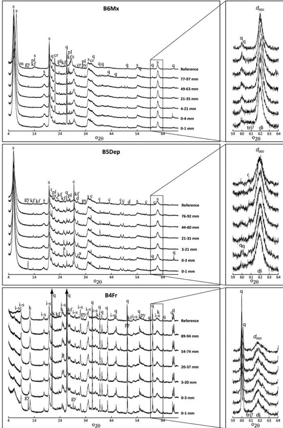
FIG. 6. XRD patterns of randomly oriented bulk samples, the minerals identified, and an enlargement of the clay minerals d_{060} region. Abbreviations: s = smectite, i-s = interstratified illite-smectite, m = illite/mica, k = kaolinite, q = quartz, pl = plagioclase, kf = K-feldspar, gy = gypsum, a = anhydrite, c = calcite, d = dolomite, cr = cristobalite, t = tridymite, py = pyrite, tri = trioctahedral, di = dioctahedral.
